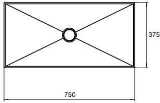
Metaphor 750 Counter Basin No taphole 9502507
