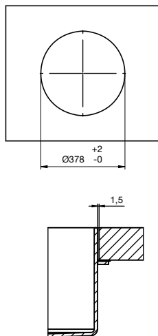
Unisono 375 Flush Mounted Basin No taphole 9506191
