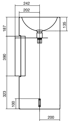
Round Washstand 400 No taphole 9502690
