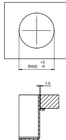
Unisono 400 Flush Mounted Basin No taphole 9506190
