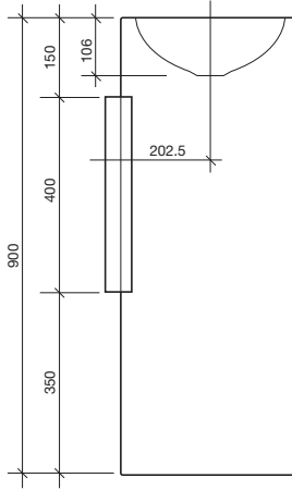
Square Washstand 325 No taphole 1805888
